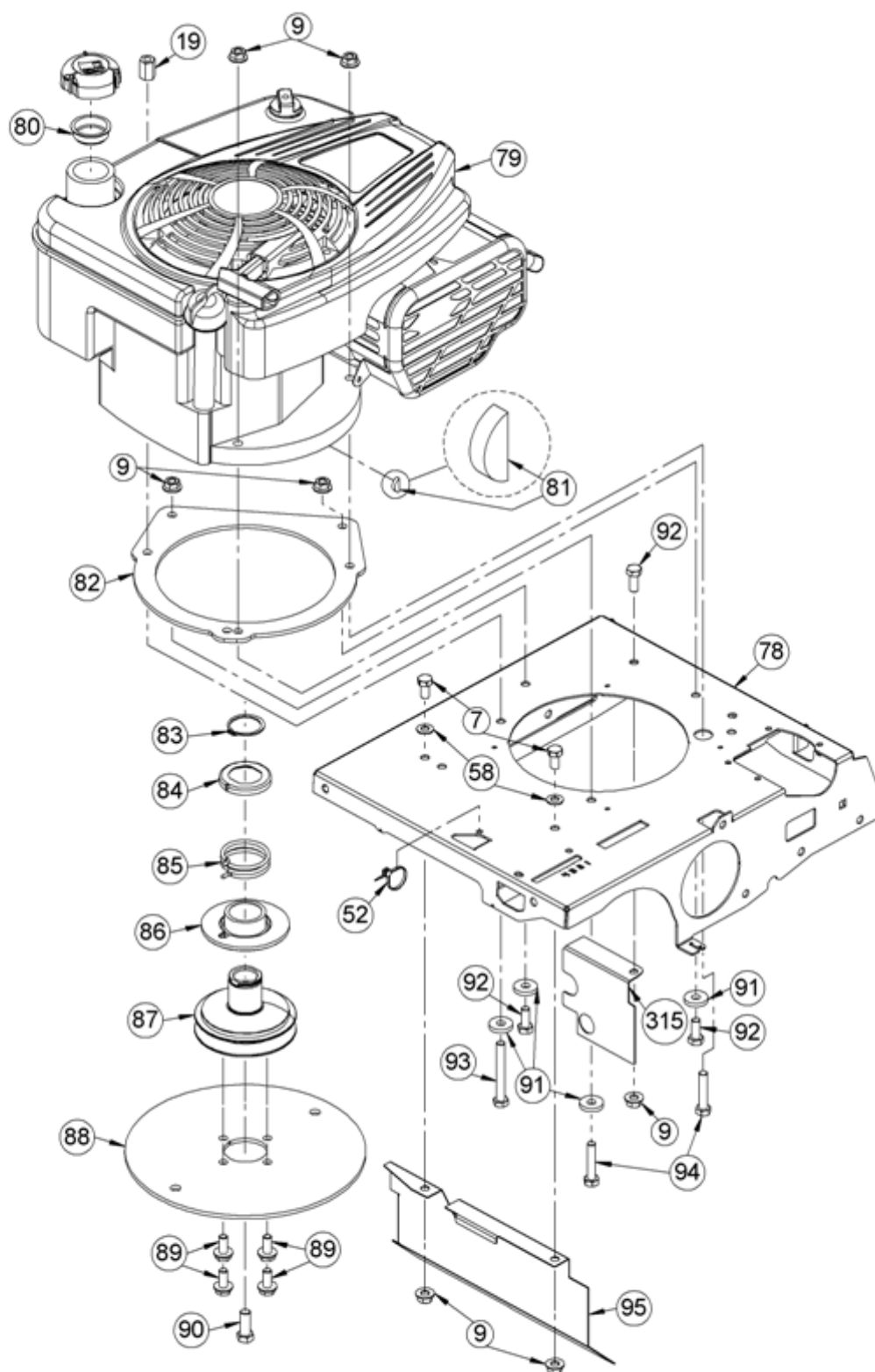
Motor AS 63 4T B&S
