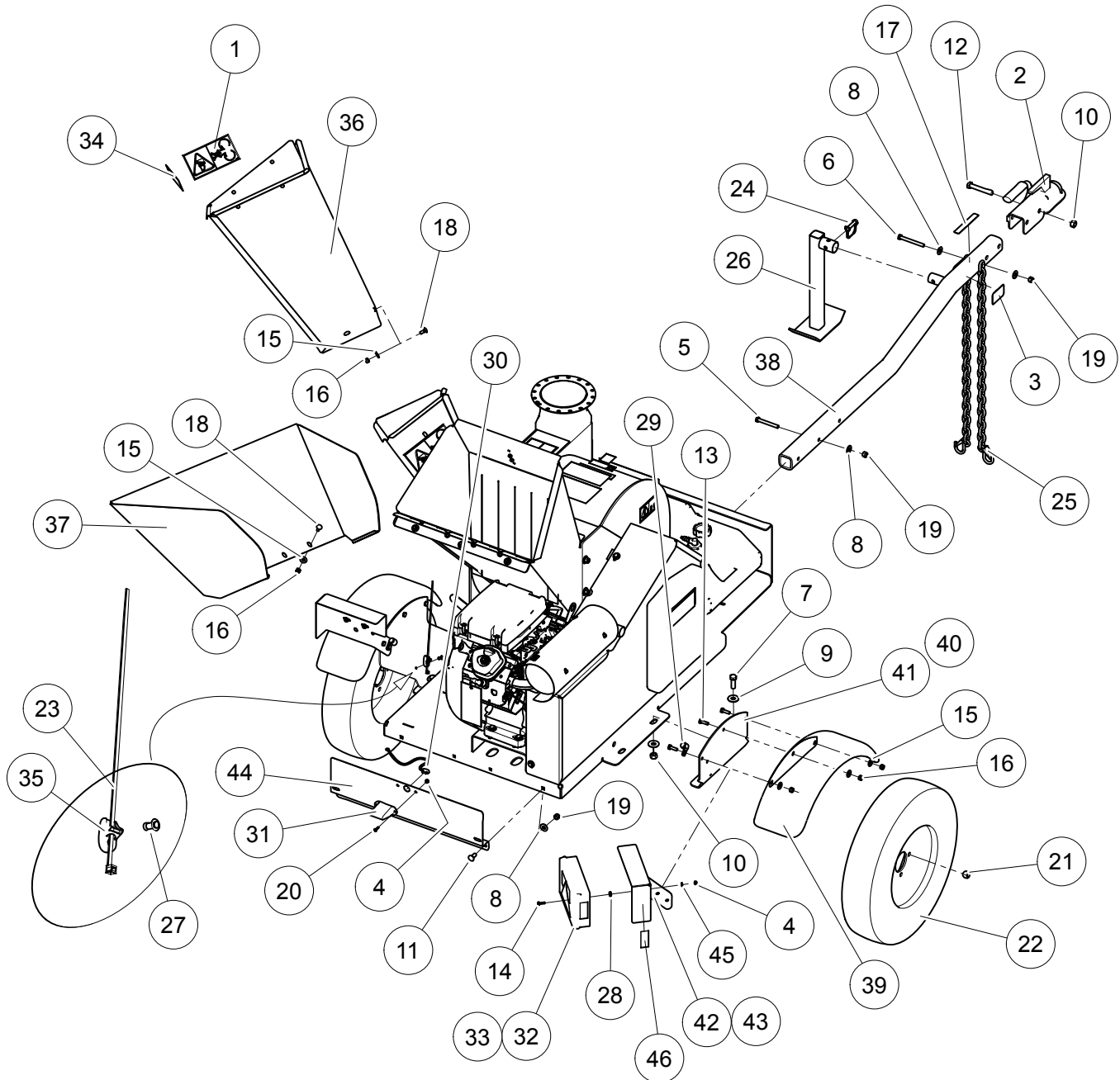
HITCH AND MISCELLANEOUS PARTS
