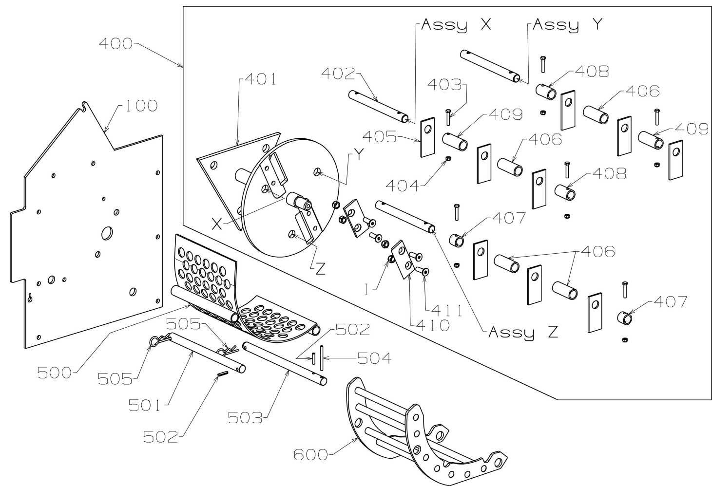
Illustration Rotor - Exploded View After assembling the flail rods,
